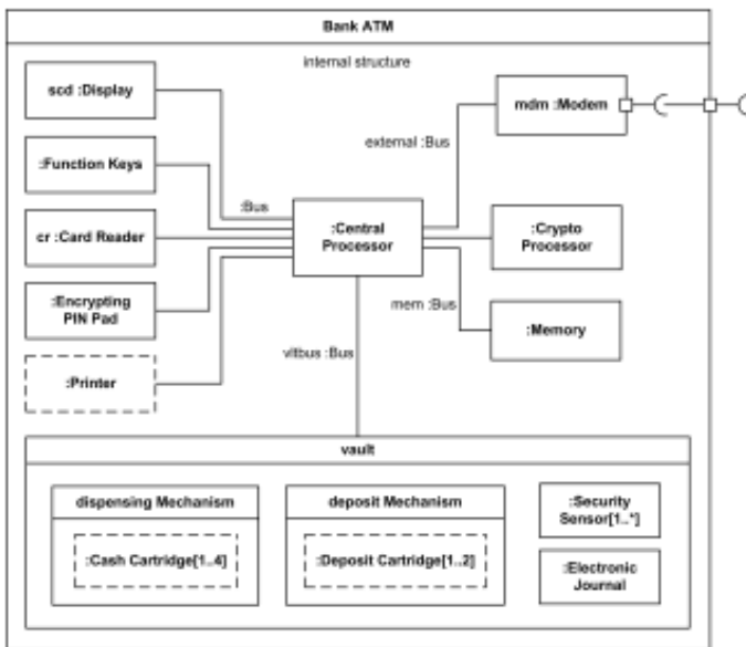
Bank ATM UML composite structure diagram example
